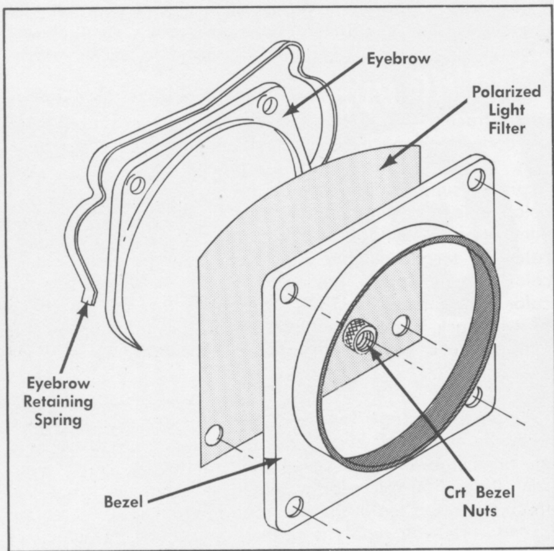
Fig. 4-2. Crt bezel and eyebrow arrangement.
