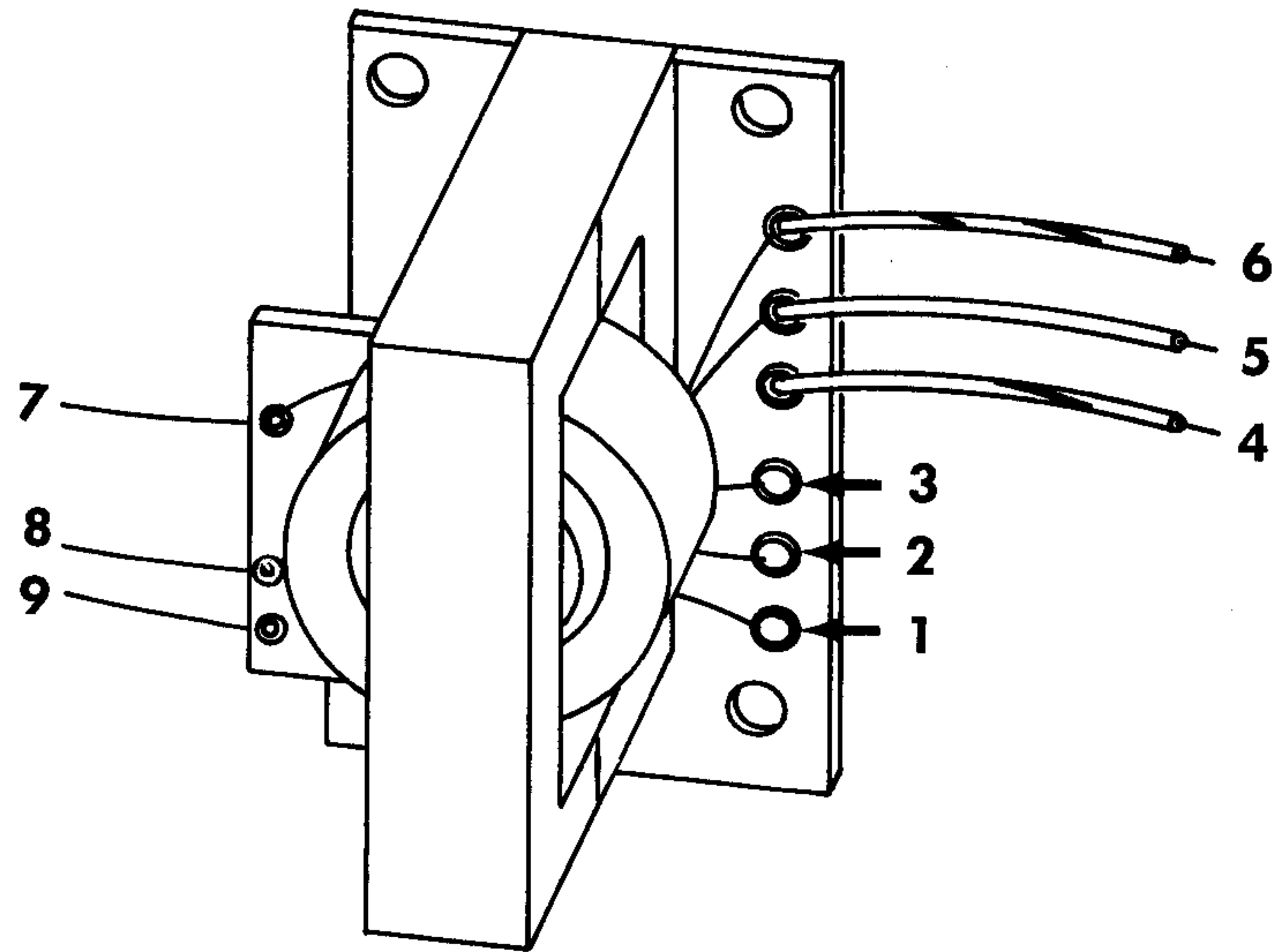
T801 TRANSFORMER DETAILS
