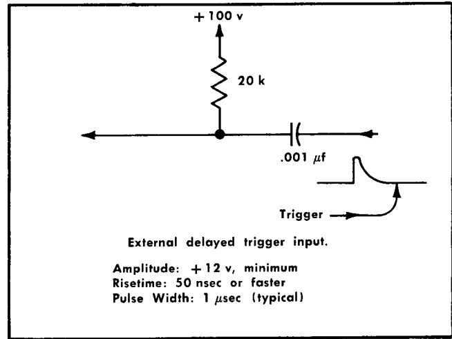
Fig. 2-1. Method of coupling an external delayed trigger into the Type 546.
