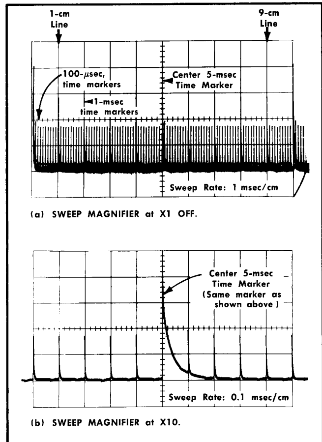
Fig. 5-7. Time marker displays.
